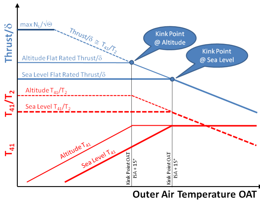
Flat rating at altitude
