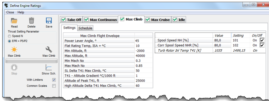
Max Climb Rating schedule input
