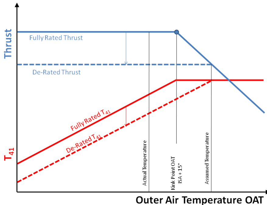
Assumed Temperature Method for De-Rating
